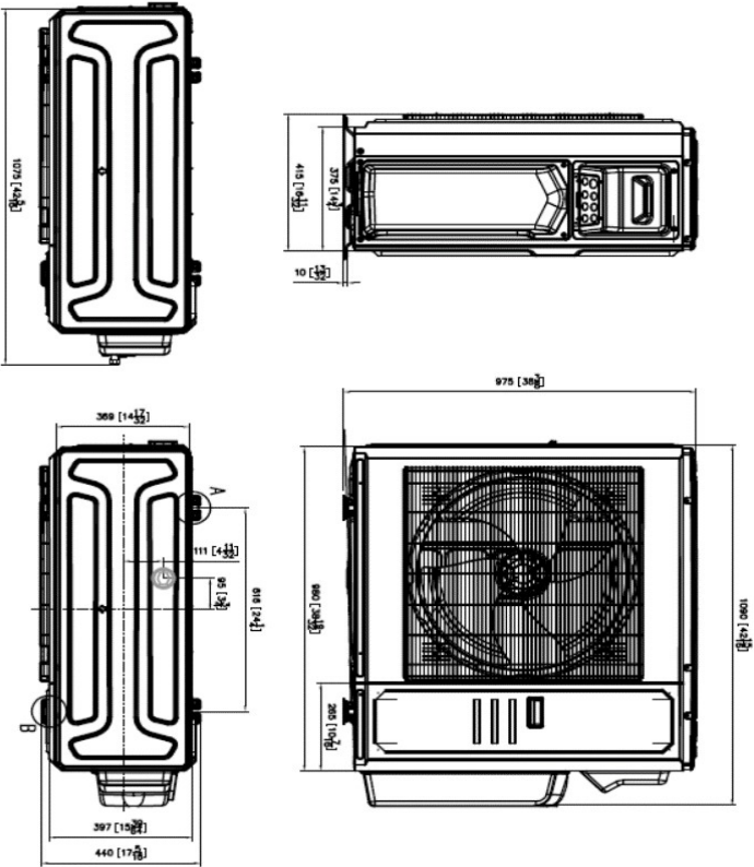
Outdoor unit dimension
